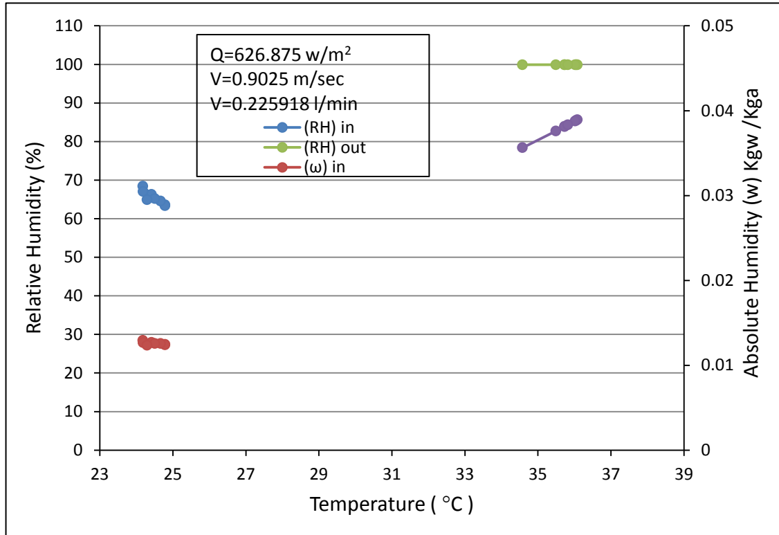
Figure (10) Day 10 Relative humidity and Absolute humidity(input+output)in humidifier
